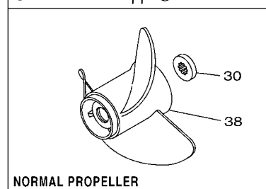
NORMAL PROPELLER
