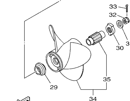
NORMAL PROPELLER
