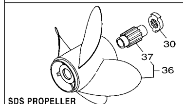
SDS PROPELLER 4 BLADE
