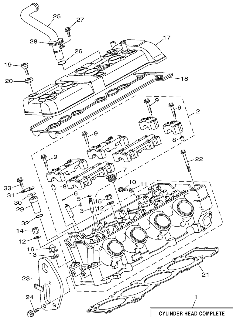
CYLINDER HEAD COMPLETE Fig. 1 CYLINDER Ref. No. 2 to 11 17 to 21 and 29 to 33 Fig. 4 VALVE Ref. No. 1 to 20 and 22 Fig.17 ELECTRICAL 2 Ref. No. 8
