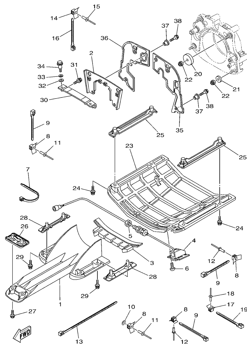
F2TD100-P170
