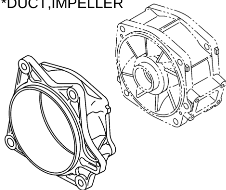
HOUSING,IMPELLER
