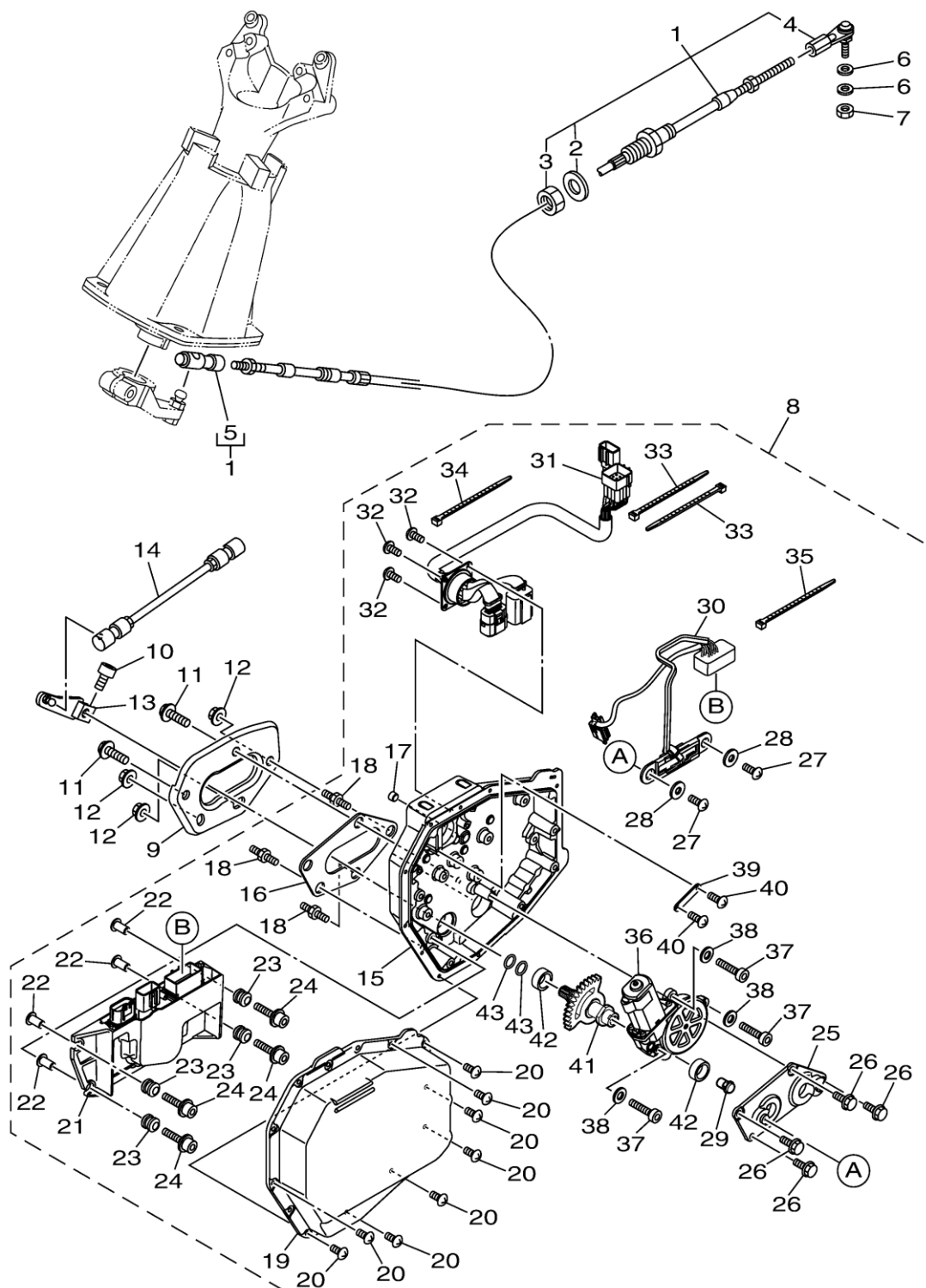
FIG. 32 CONTROL CABLE SECTION 3. ILLUSTRATION CORRECTION
